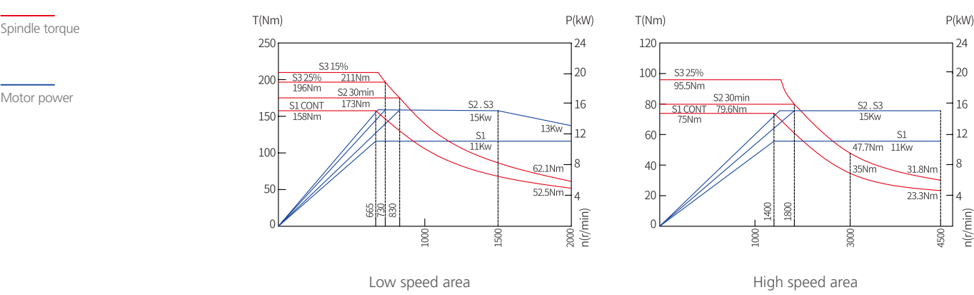
HTC200 II Power & Torque Diagram
