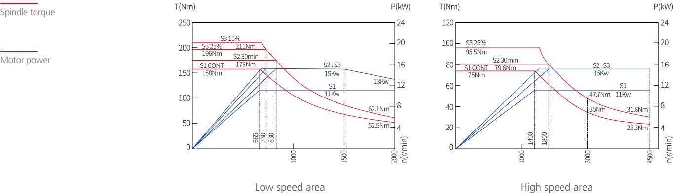
HTC150 II Power & Torque Diagram
